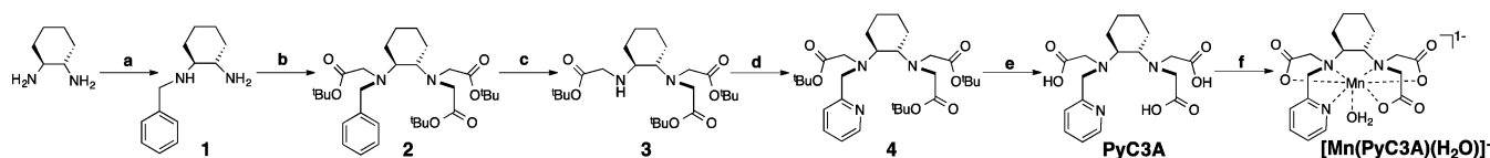
Scheme 1. Synthesis of [\text{Mn}(\text{PyC3A})(\text{H}_2\text{O})]^{-4}
