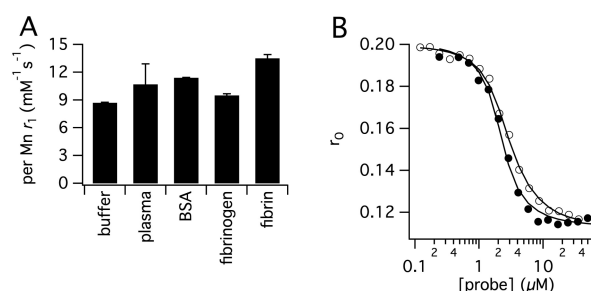
Figure 4. (A) r_1 of Mn-FBP measured in pH 7.4 Tris buffer, bovine blood plasma, 4.5 wt %/v BSA, human fibrinogen and human fibrin gel at 1.4T, 37 °C. The 60% r_1 increase in the presence of fibrin gel is the result of the reduction in Mn-FBP tumbling rate upon protein binding. (B) Fluorescence polarization anisotropy of fluorescein labeled fibrin binding peptide in DD(E) solution as a function of added Mn-FBP (filled circles) or EP2104R (open circles) to determine K_i to DD(E).
