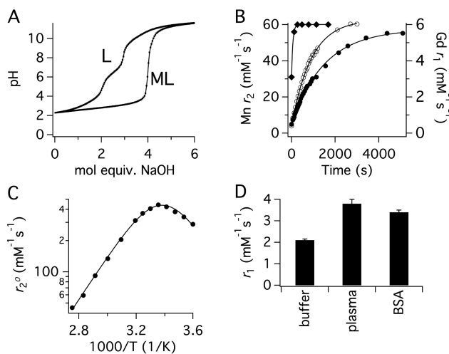
Figure 1. (A) pH titration of PyC3A·TFA in the absence (L) and presence (ML) of 1 equiv of MnCl 2 at 25 °C, I = 0.15 M NaCl. (B) Transmetalation of 1 mM [\text{Gd}(\text{DTPA})(\text{H}_2\text{O})]^{2-} (filled diamonds), [\text{Mn}(\text{CDTA})(\text{H}_2\text{O})]^{2-} (open circles) or [\text{Mn}(\text{PyC3A})(\text{H}_2\text{O})]^- (filled circles) by 25 mM Zn 2+ monitored by relaxivity change as a function of time in 50 mM pH 6.0 MES buffer, 37 °C, 1.4 T. (C) H 2 17 O transverse relaxivity in the presence of [\text{Mn}(\text{PyC3A})(\text{H}_2\text{O})]^- as a function of temperature. Solid lines are fits to the data. (D) r_1 of [\text{Mn}(\text{PyC3A})(\text{H}_2\text{O})]^- measured in pH 7.4 Tris buffer, bovine blood plasma, and 4.5 wt %/v bovine serum albumin (BSA) at 1.4 T, 37 °C.
